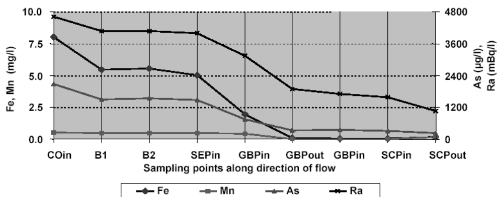
Figure 4: Contaminant concentration at sampling points along direction of flow through wetland
