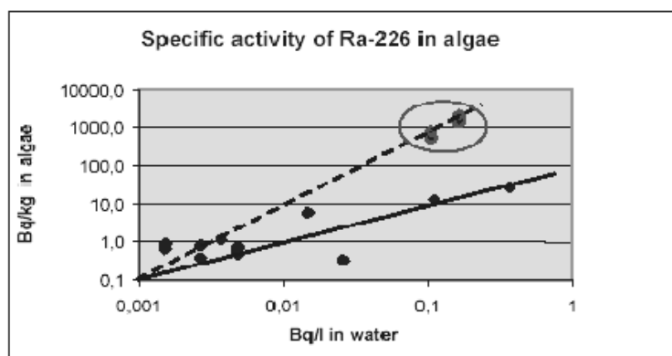
Figure 5: Specific activity of Ra-226 in algae
