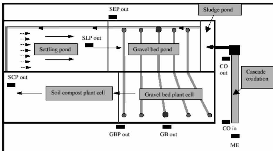
Figure 2: Schematic layout of the experimental constructed wetland Poehla site
