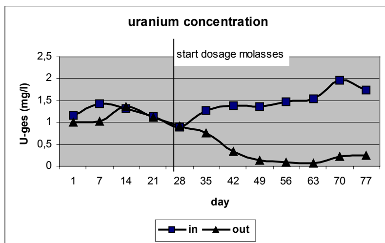
Figure 9: Uranium concentration in the input and discharge of the planted part of the facility
