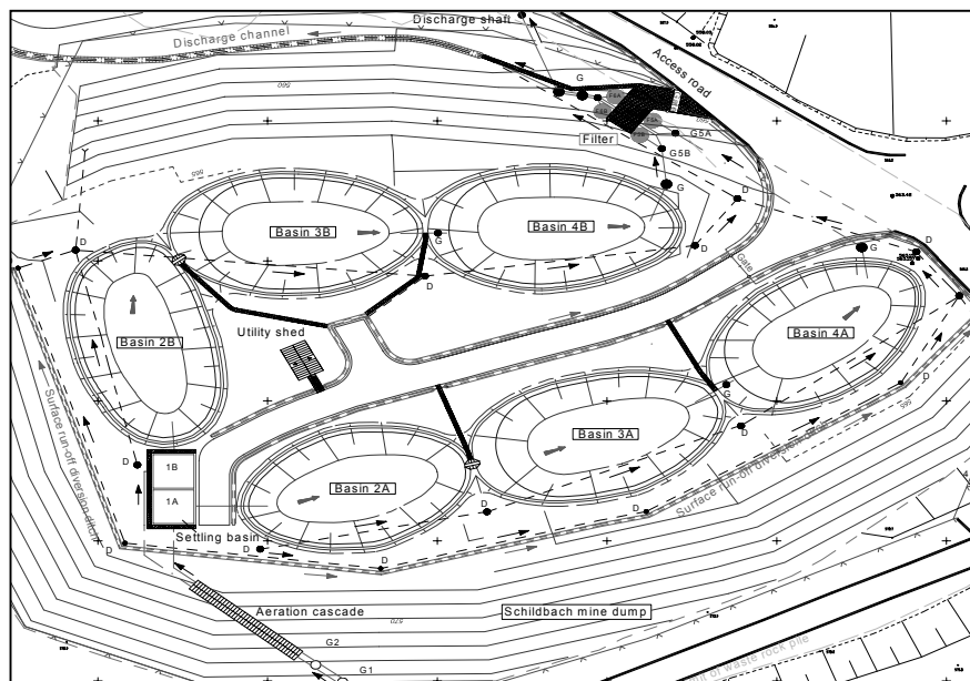
Figure 6: Schematic layout of the constructed wetland Poehla site
